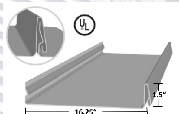
Wagler Standing Seam Profile
