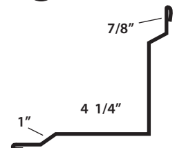
22 Inside Corner
