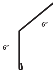
20 Gambrel Trim
