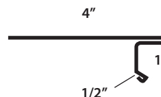
21 Residential Eave
