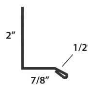
20 Gambrel Trim
