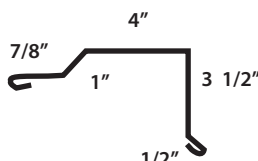
19 Gable Flashing
