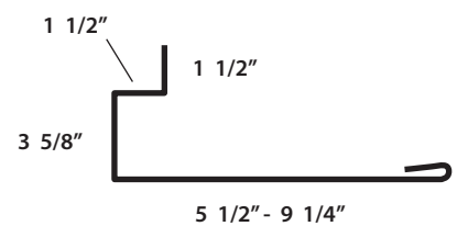
21 Residential Eave
