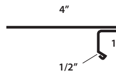
21 Residential Eave
