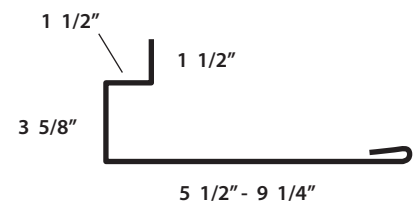
21 Residential Eave
