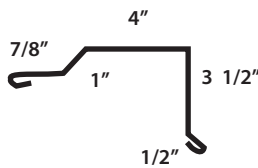
19 Gable Flashing
